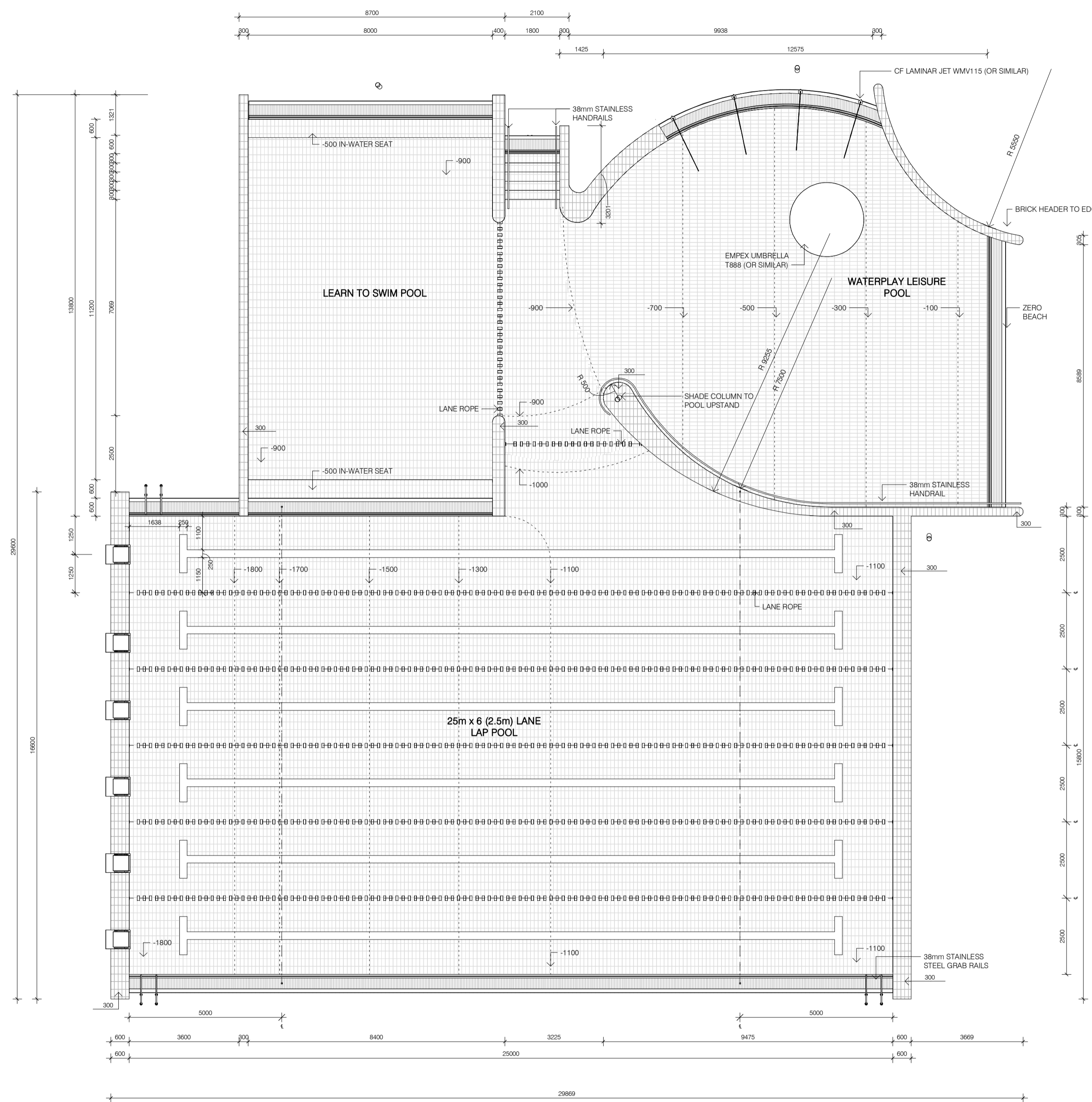
1 PROPOSED POOL LAYOUT A105 1 : 100
